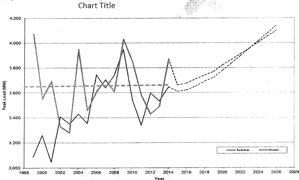
Figure 7: Portland General Electric's Historic & Projected Seasonal Peak Load (Projection is for a 1-in-3 Loading Condition)
