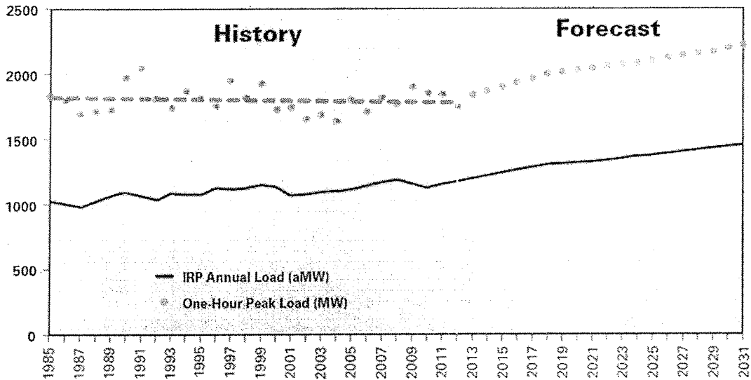
FIGURE 5: LOAD HISTORY AND 2012 IRP FORECAST (WITH NO NEW PROGRAMMATIC CONSERVATION)
